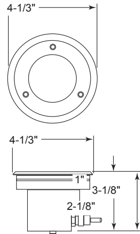
PVC well housing
