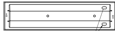
2X 1/2" Hole Knockouts for electrical connections.
